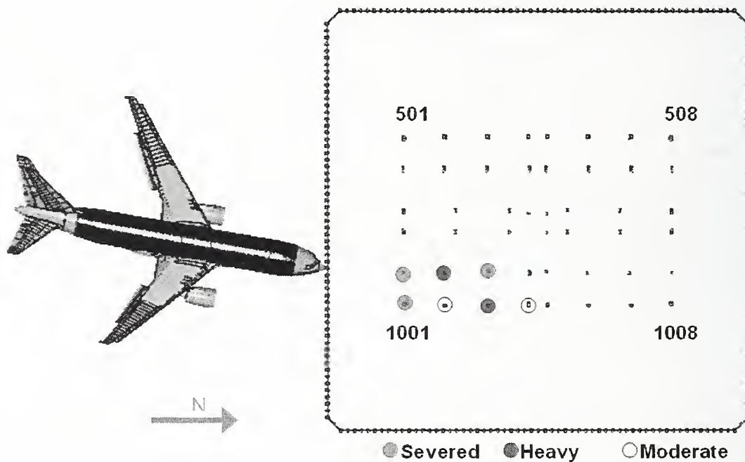
Figure 9–97. Summary of core column damage for the less severe WTC 2 impact.
