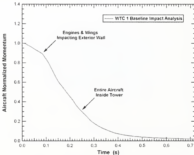
Figure 9–6. Normalized aircraft momentum for the WTC 1 base case impact.
