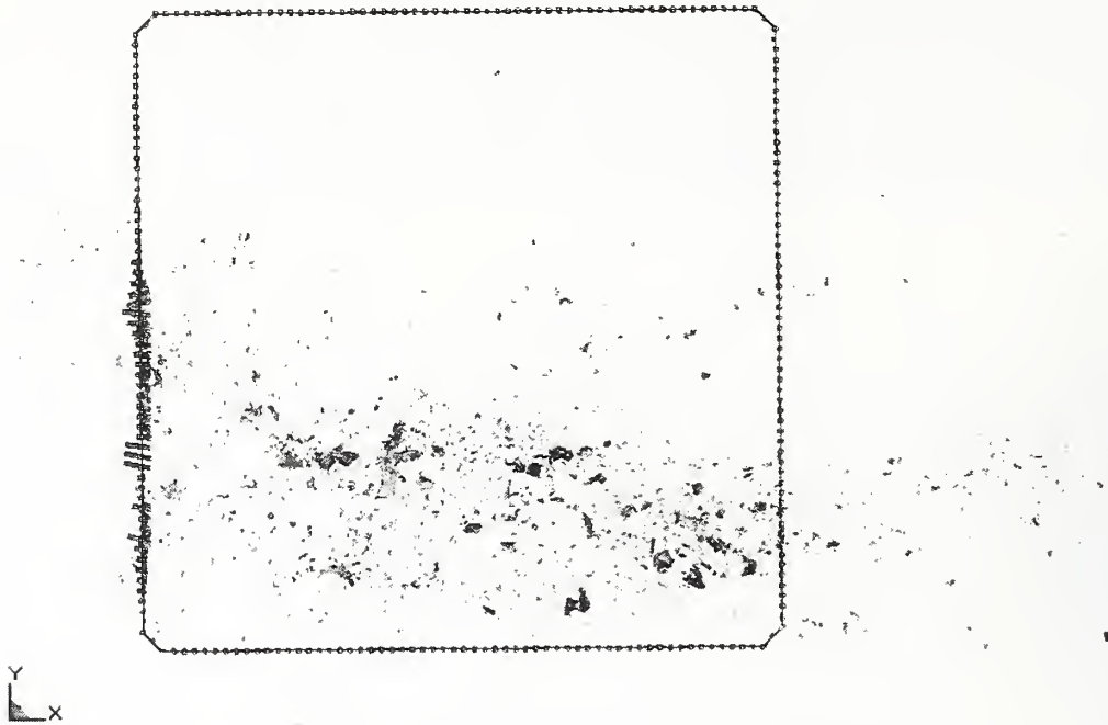
(a) Calculated aircraft debris ( t = 0.62 s)
