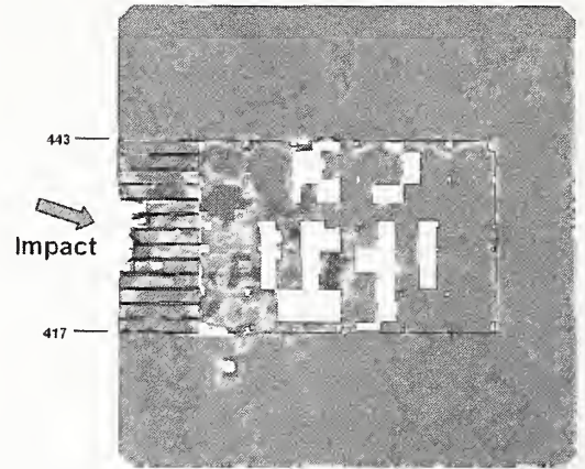
(b) Floor 79 slab damage
