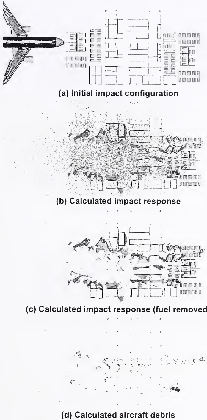
Figure 9–22. Calculated floor 96 contents, fuel, and aircraft debris distribution.
